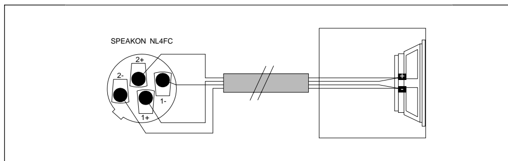
Figure 3-2 ES 10 4-terminal loudspeaker connection.
