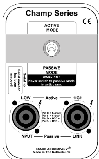
SpeakON connectors and active/passive switch of the C29
