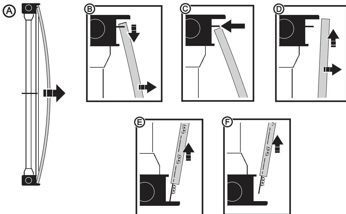
Figure 21: Removing an LED tube
