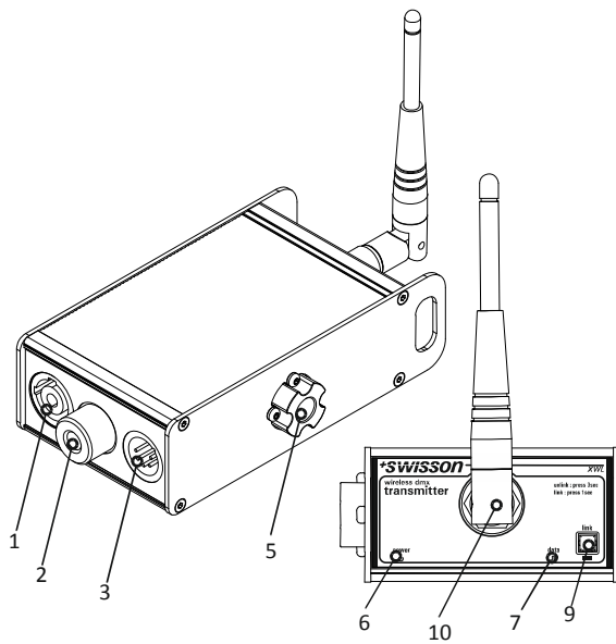
XWL-T wireless DMX transmitter
