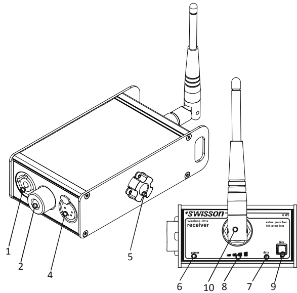
XWL-R wireless DMX receiver
