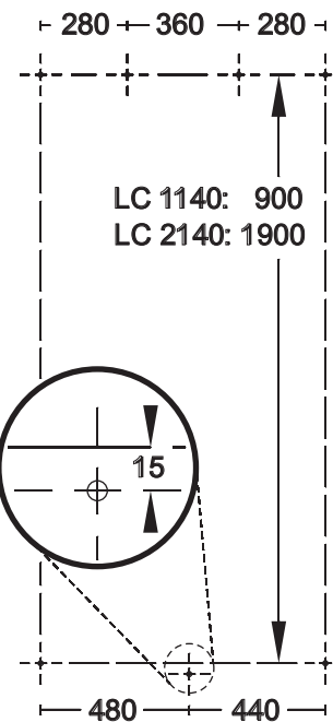
LC Video Wall Diffuser mounting hole pattern
