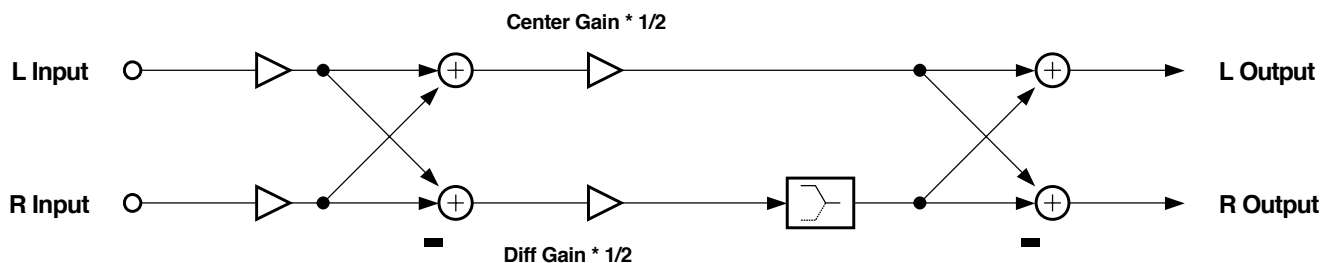
Block diagram of Stereo Image algorithm
