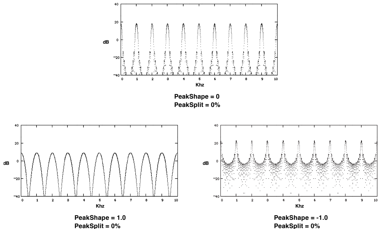
Response of Pitcher with PkShape settings at 0, -1.0, and 1.0.
