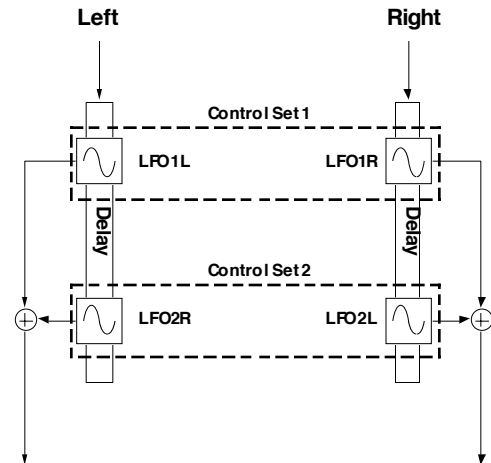
Fig. 4 — LFO control in Link2Tap mode
