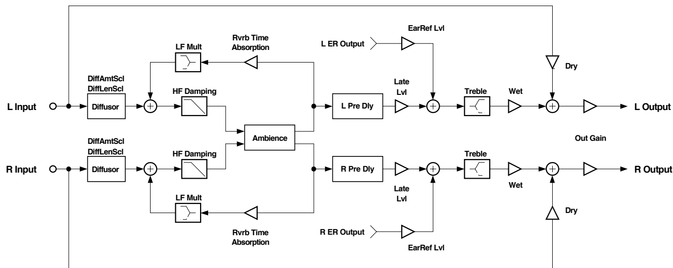
Signal flow of Classic Verb and Classic Place
