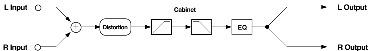
Block diagram of MonoDistort + EQ
