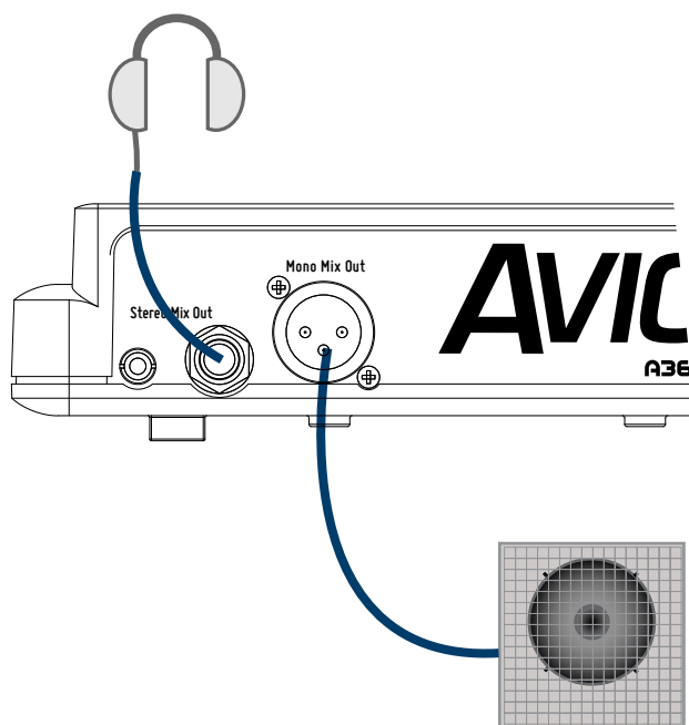
Headphones and a subwoofer are connected to the A360.
