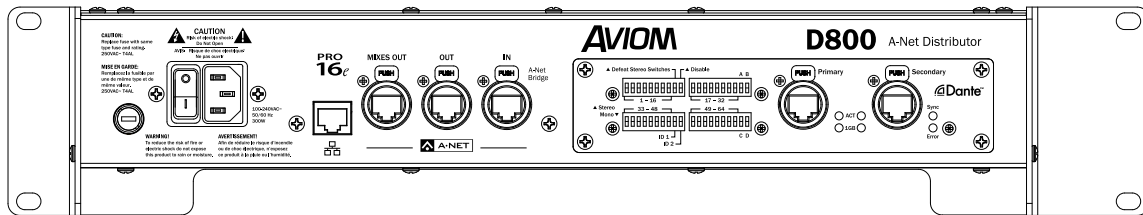
D800-Dante A-Net Distributor rear panel
