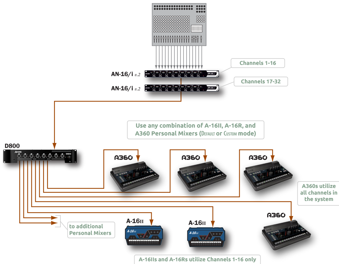
A 32-input personal mixing system with A-16II and A360 Personal Mixers
