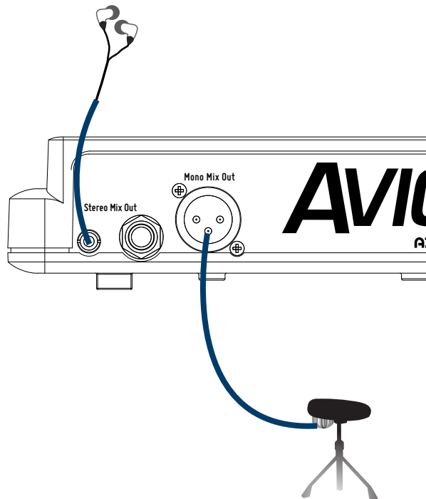
The A360 is shown connected to earbuds plus a drum throne shaker device.
