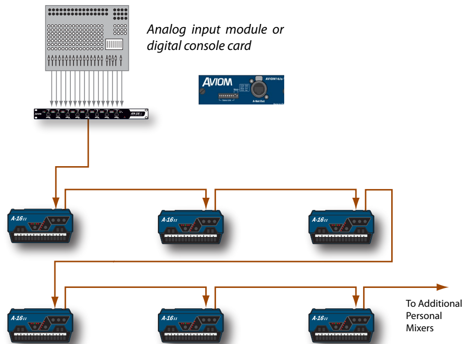
A typical daisy chained Pro16 personal mixing system with six A-16II mixers is shown.
